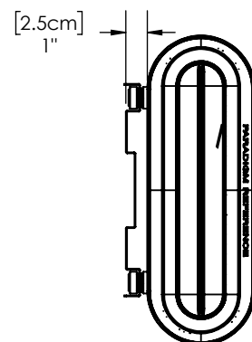
SIDE VIEW (with Mounting Bracket)
