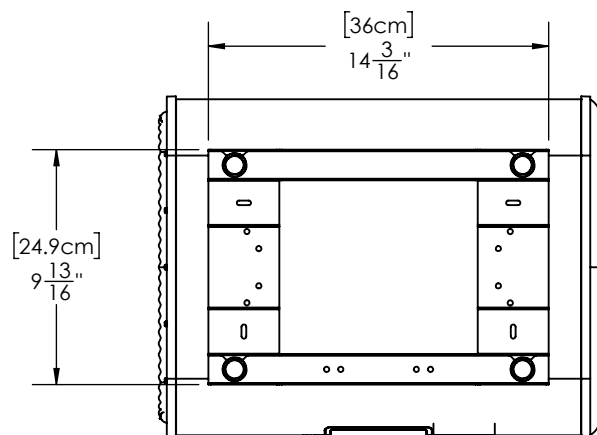
BACK VIEW (with Mounting Bracket)
